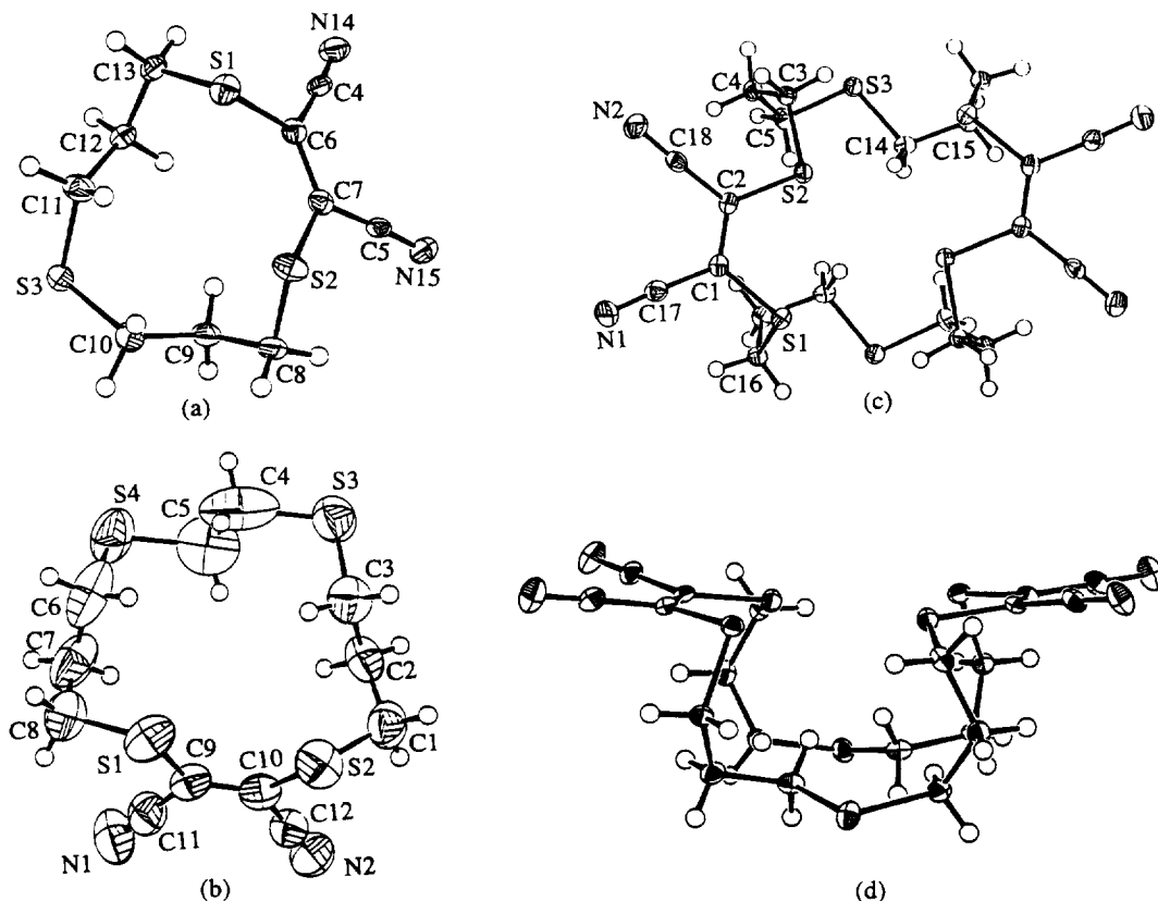
Figure 1: ORTEP representations of compounds of 5 (a), 8 (b) and 6 (c,d).
